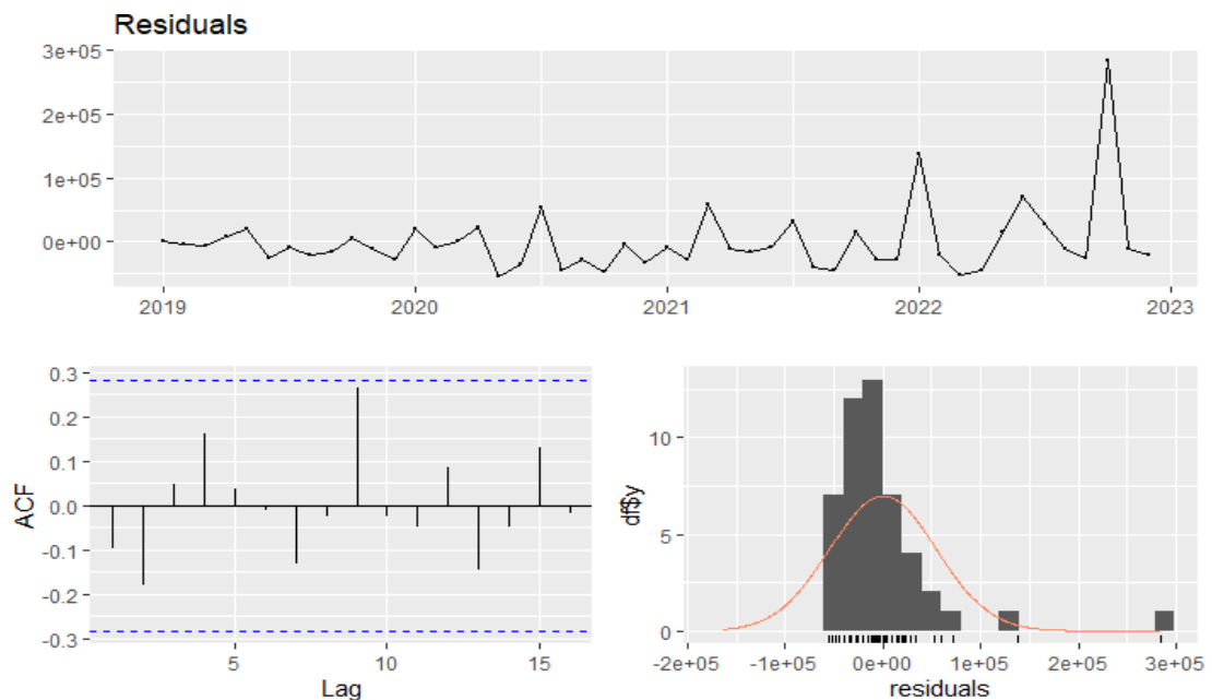
Figure 16: Auto-Arima Residuals
