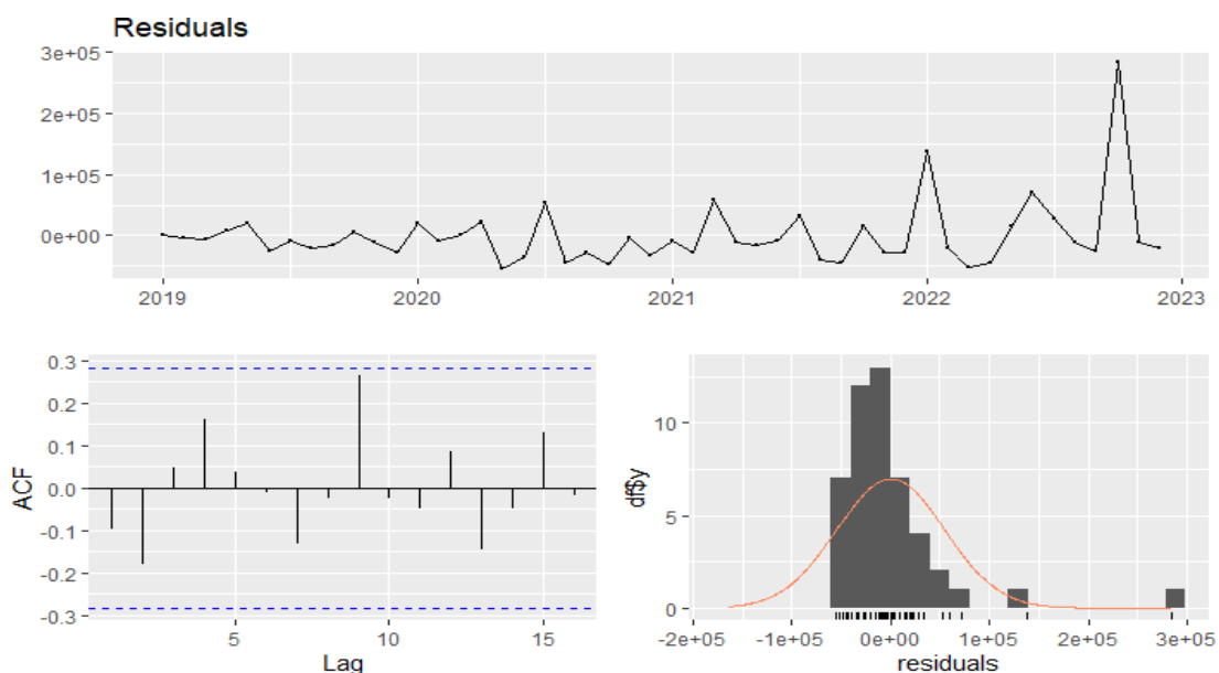
Figure 10: SES Residuals
