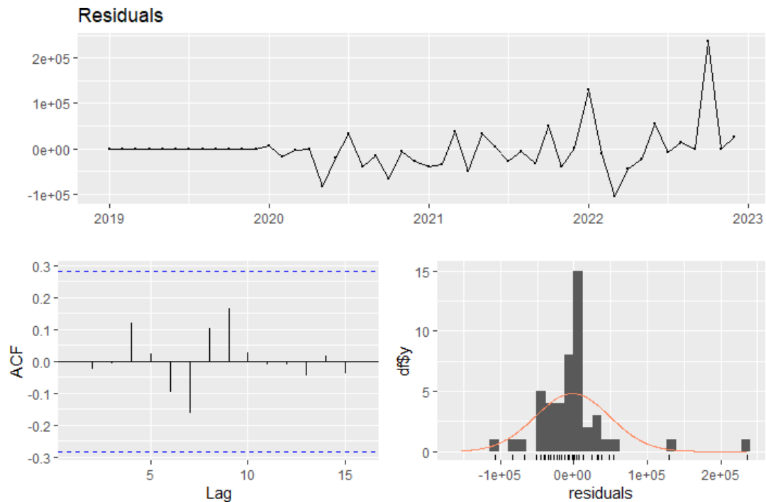
Figure 18: SARIMA Residuals
