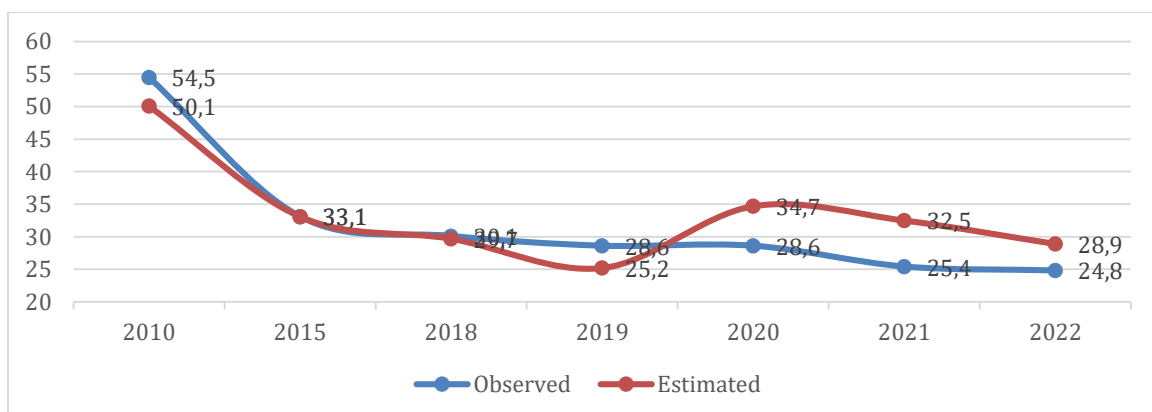
Figure 5. Distribution of observed and estimated poverty in Tajikistan Note: (compiled by the authors based on modeling in Gretl software)
