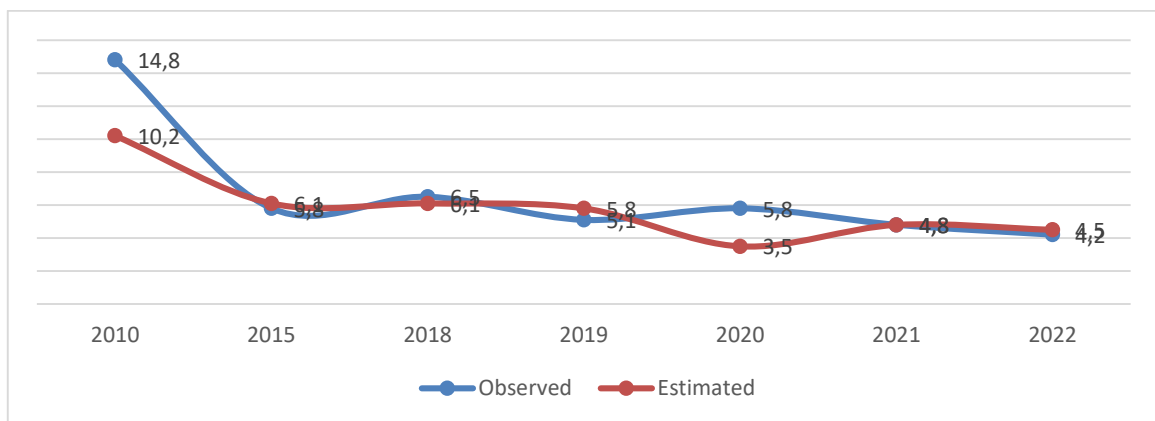
Figure 2. Distribution of observed and estimated poverty in Kazakhstan Note: (compiled by the authors based on modeling in Gretl software)
