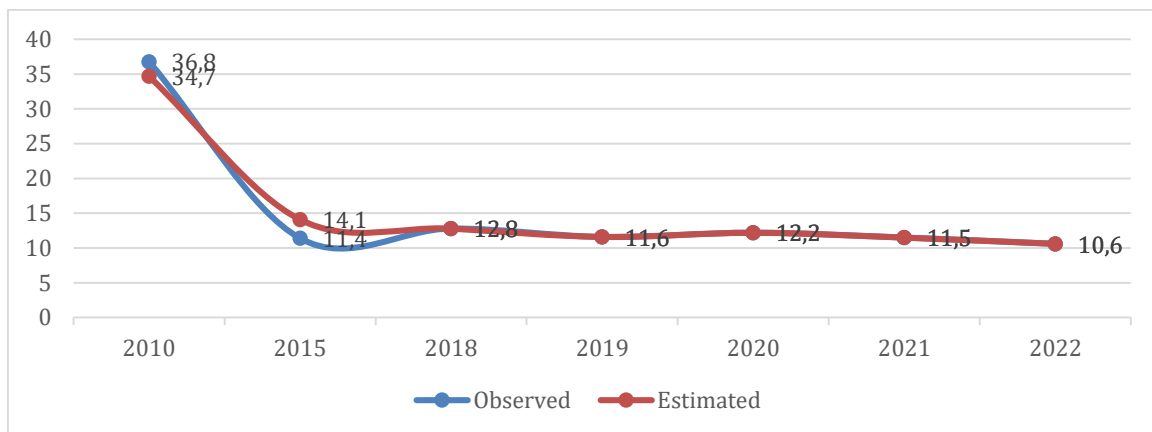
Figure 4. Distribution of observed and estimated poverty in Uzbekistan Note: (compiled by the authors based on modeling in Gretl software)
