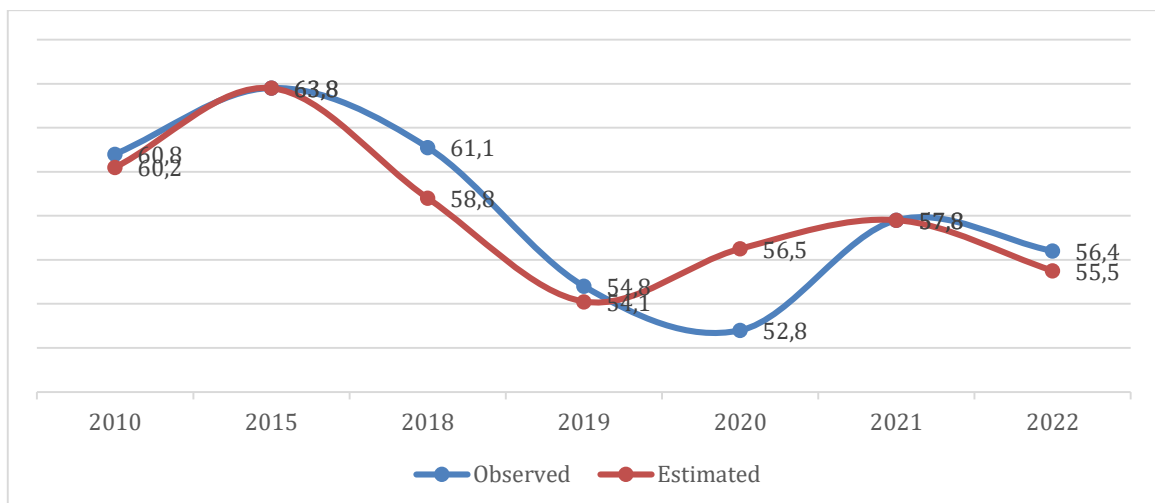
Figure 3. Distribution of observed and estimated poverty in Kyrgyzstan Note: (compiled by the authors based on modeling in Gretl software)
