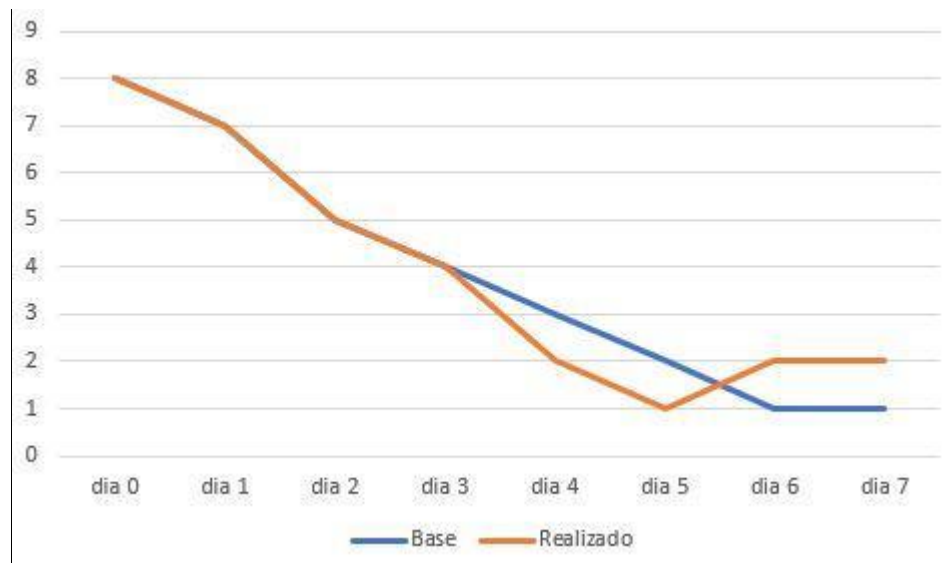
Figura 5: Burndown Sprint 3
